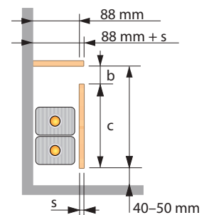
Plintverwarming IIIa Classic
