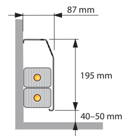
Plintverwarming IIIa Delta
